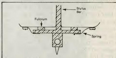
Fig. 2. Form of mounting used on Decca Telesmatic.
